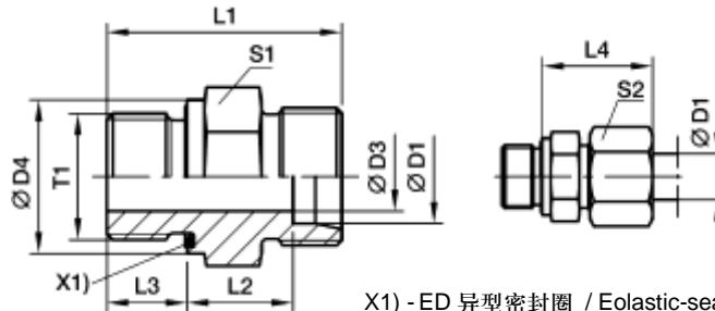
X1) - ED 异型密封圈 / Elastic-sealing (ED)
